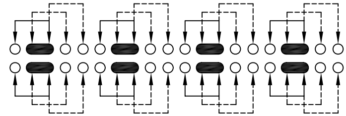
SCHEMATIC (SHORTING)
